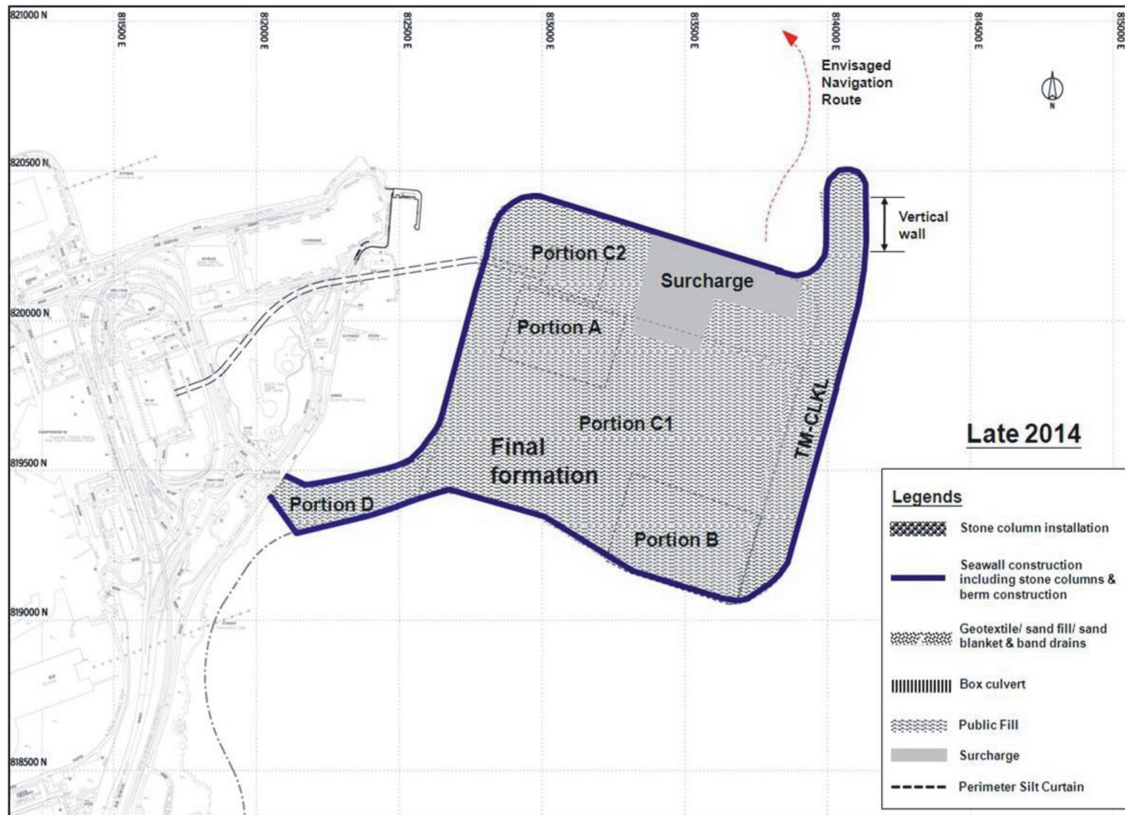
Figure 20 - Outline of Construction Sequence (Sheet 9 of 10)
